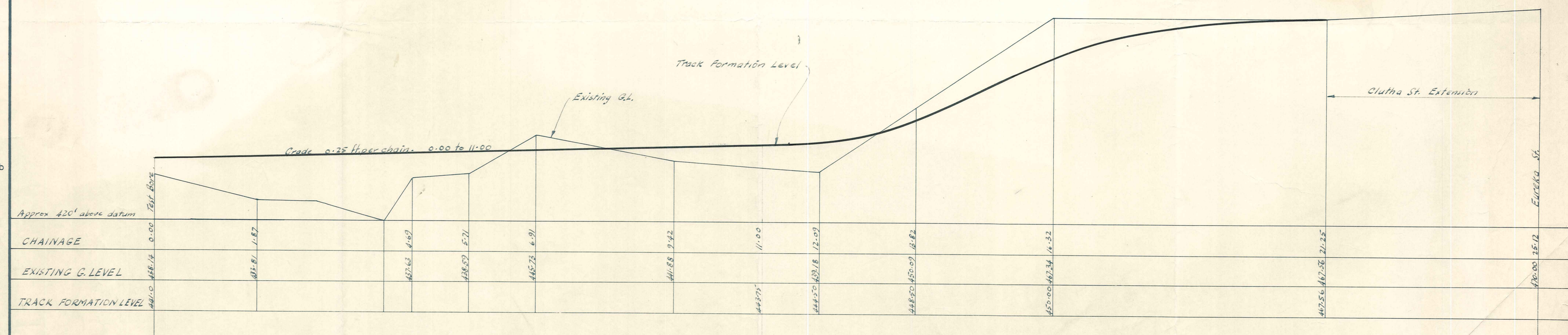
LONG SECTION Scales: - Vertical - 10 ft. to 1 in. Horizontal - 1 in. to 1 in.
