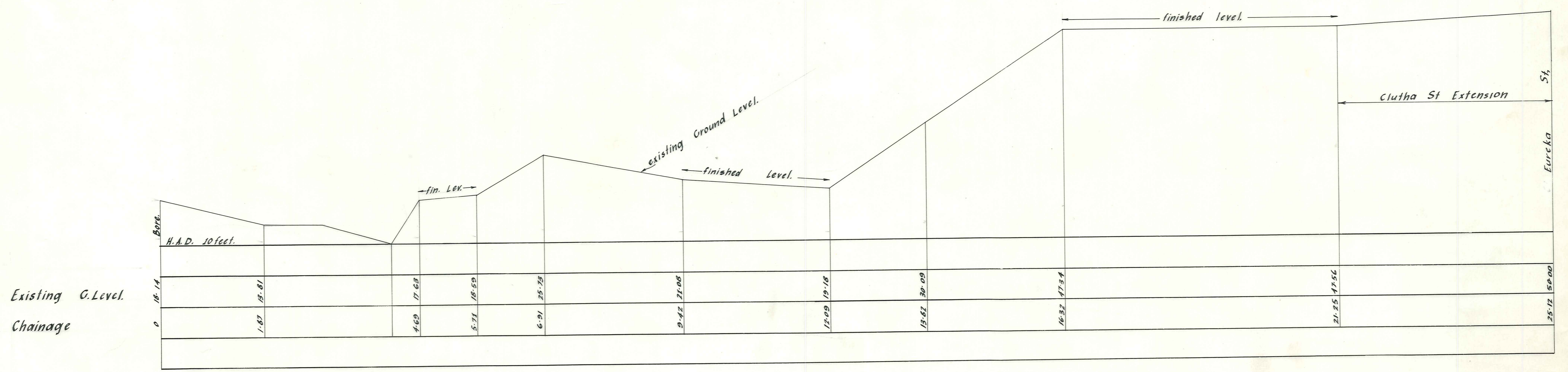
—LONGITUDINAL SECTION— Vertical: 10 feet to linch. Scales: Horizontal: 1chain to linch.
