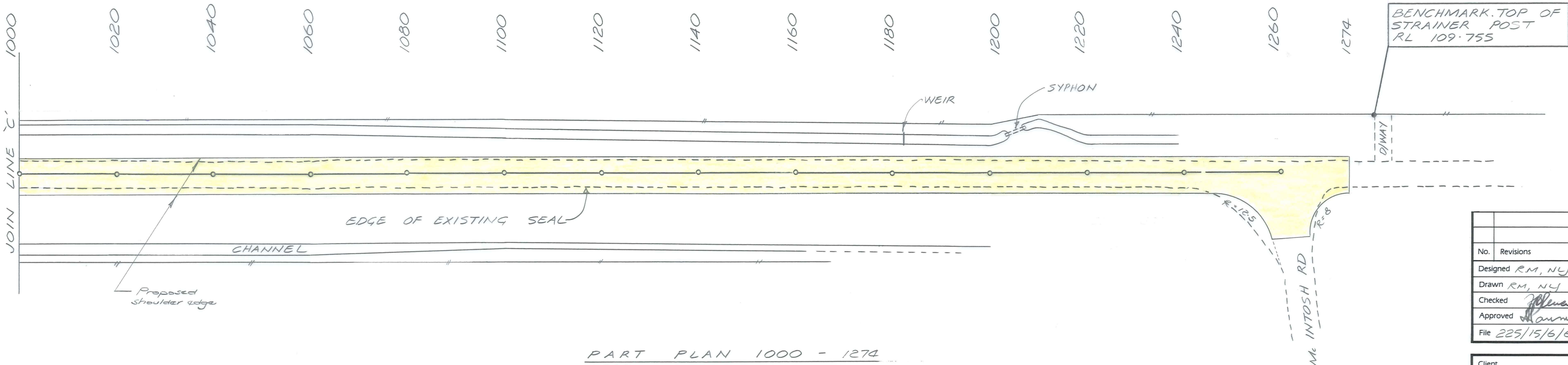
PART PLAN 1000 - 1274 1:500
