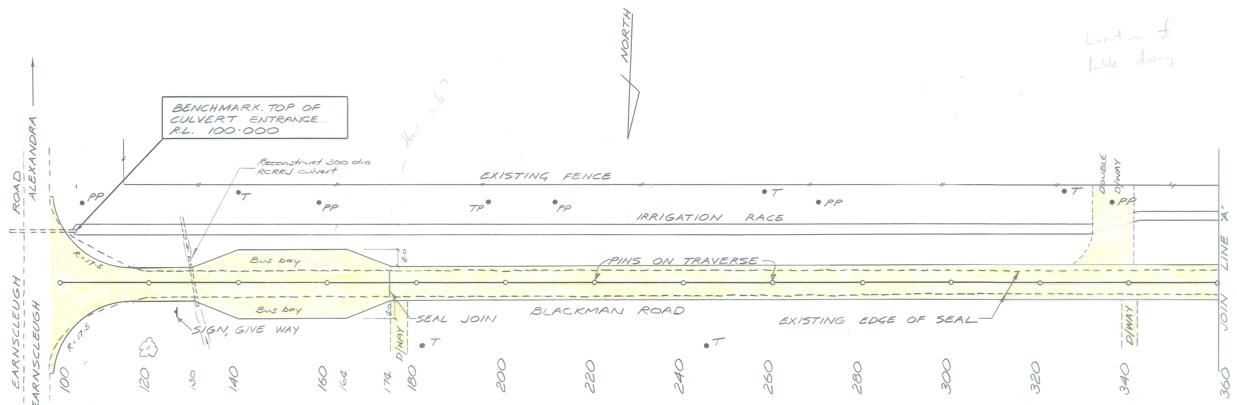
PART PLAN 100 - 360 1:500
