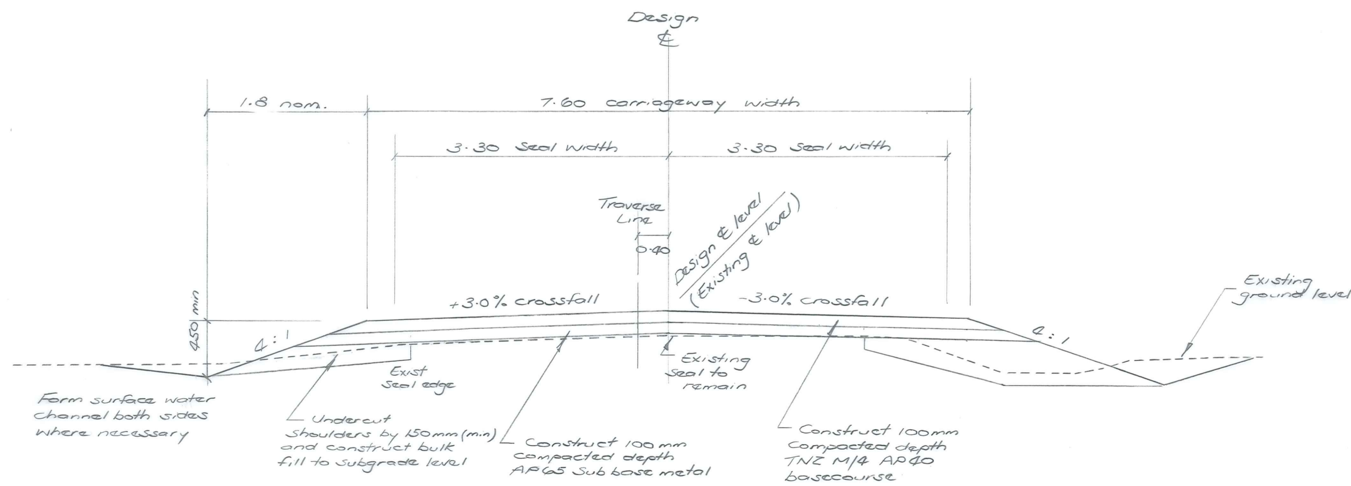
TYPICAL CROSS SECTION
