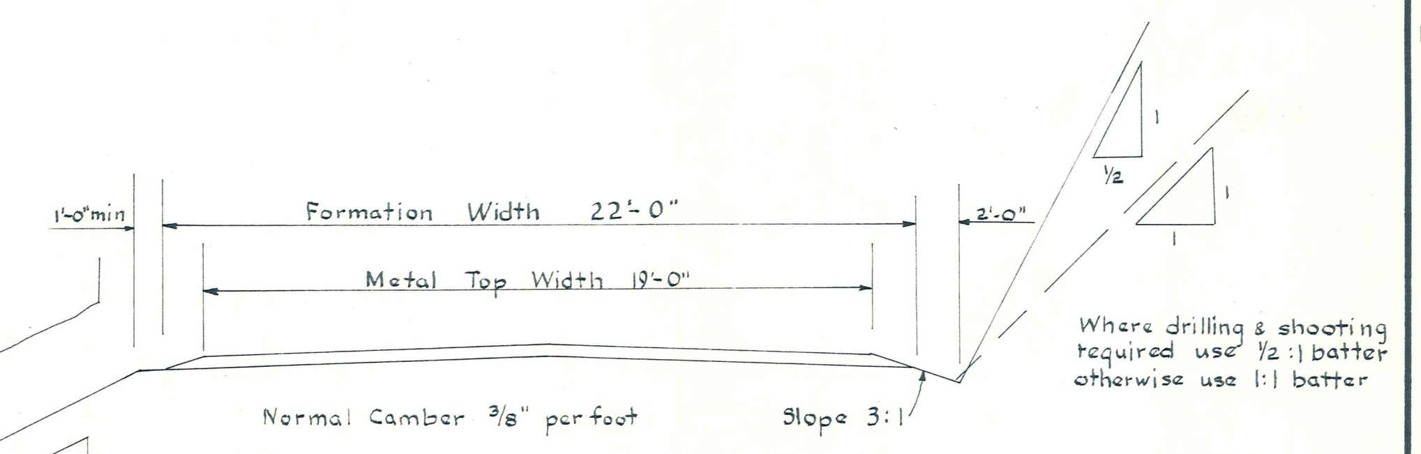
TYPICAL X-SECTION
