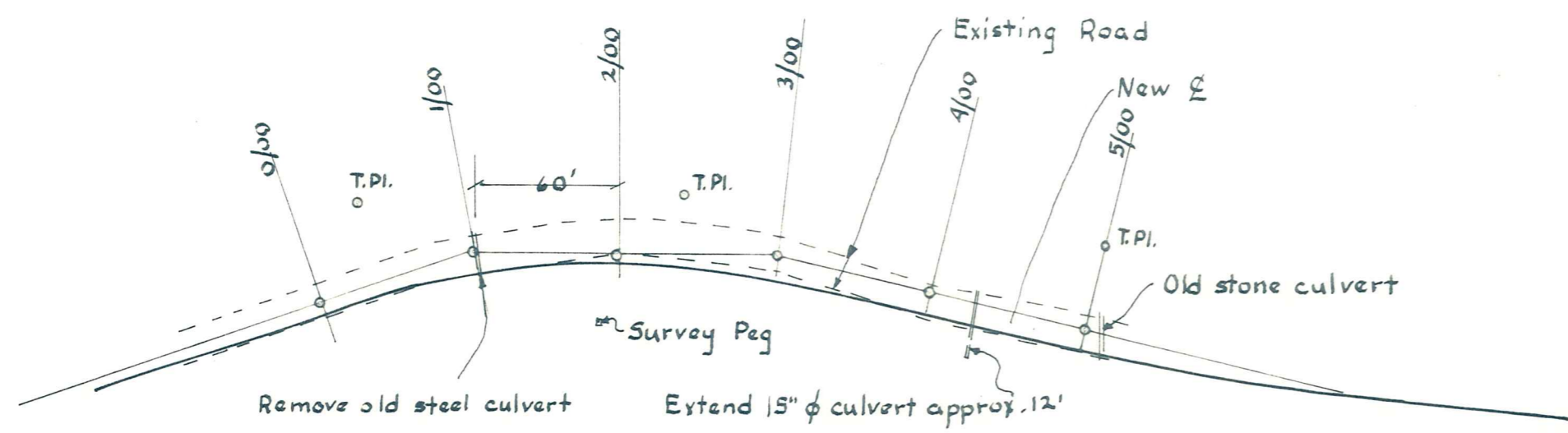
PLAN Scale - 1 ch. to 1 inch
