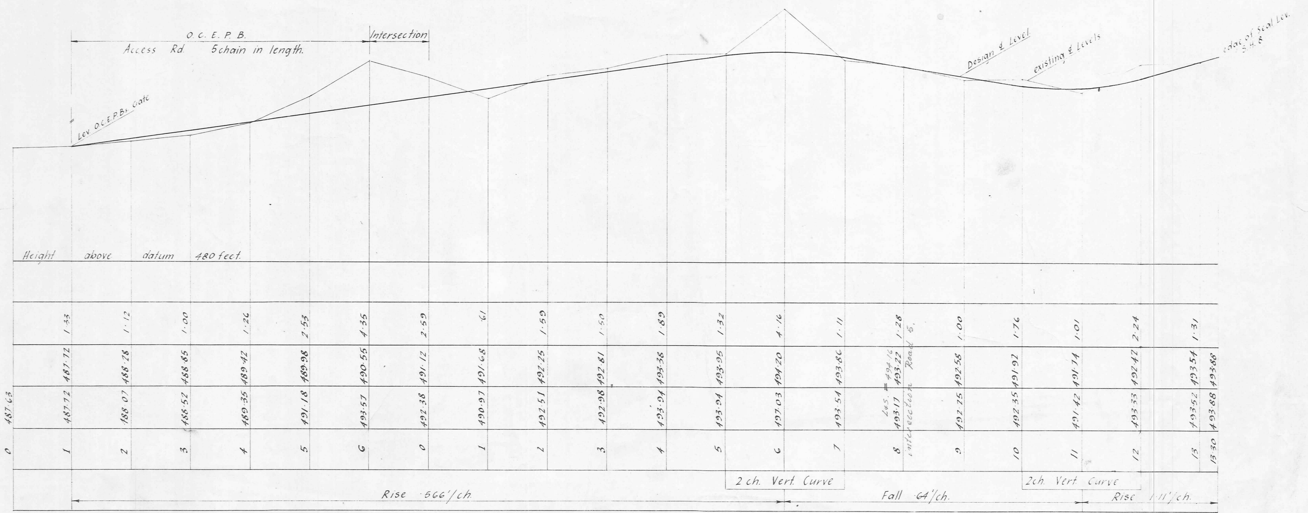
—LONGITUDINAL SECTION— Vertical: 4ft. to lin. Scale: Horizontal: 1ch to lin.
