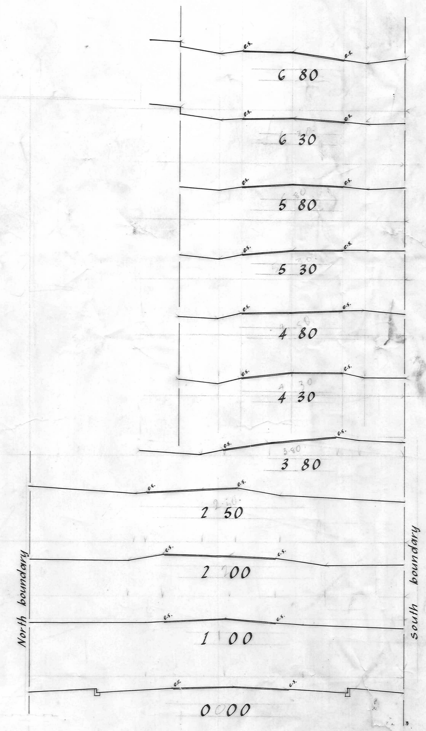
CROSS SECTIONS Vertical: 5 ft. to lin. Scales: Horizontal: 10 ft. to lin. ALEXANDRA BOROUGH COUNCIL FOX & KERRY ST. RE-ALIGNMENT.
