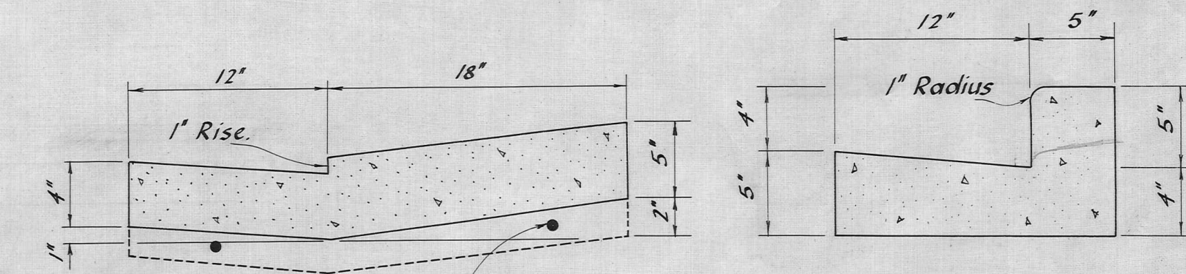
SECTION OF DISH CHANNEL & KERB & CHANNEL Scale: 1 1/2 inches to 1 foot.
