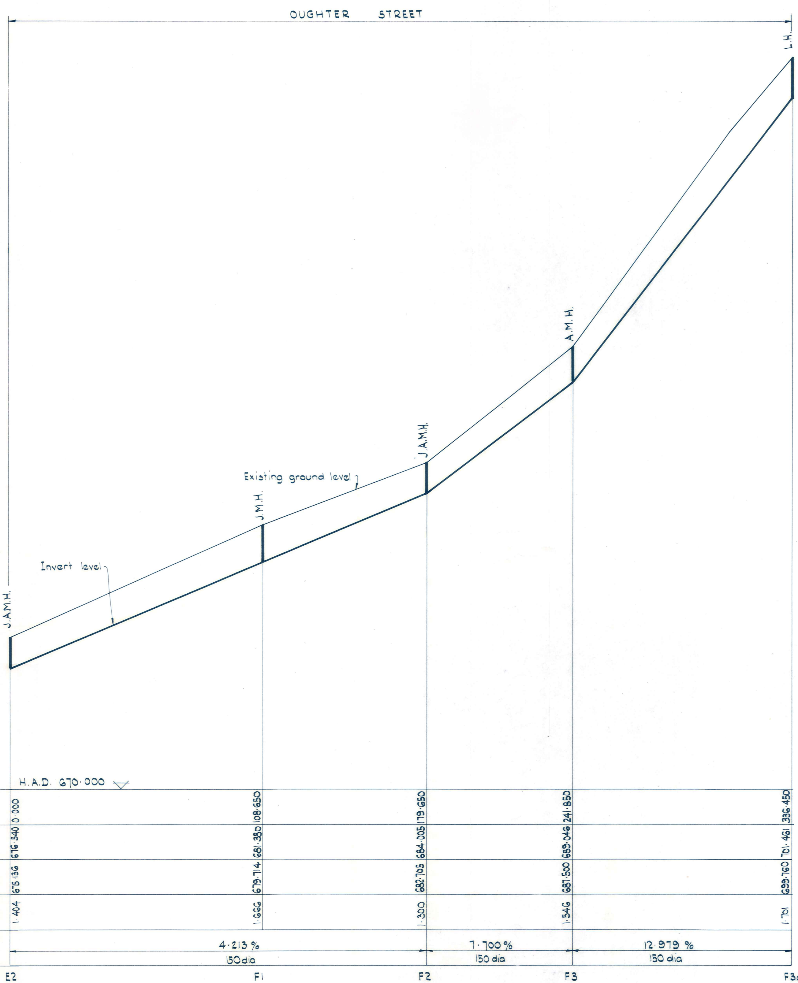
PROFILES Scales - Horizontal 1:1000 Vertical 1:100
