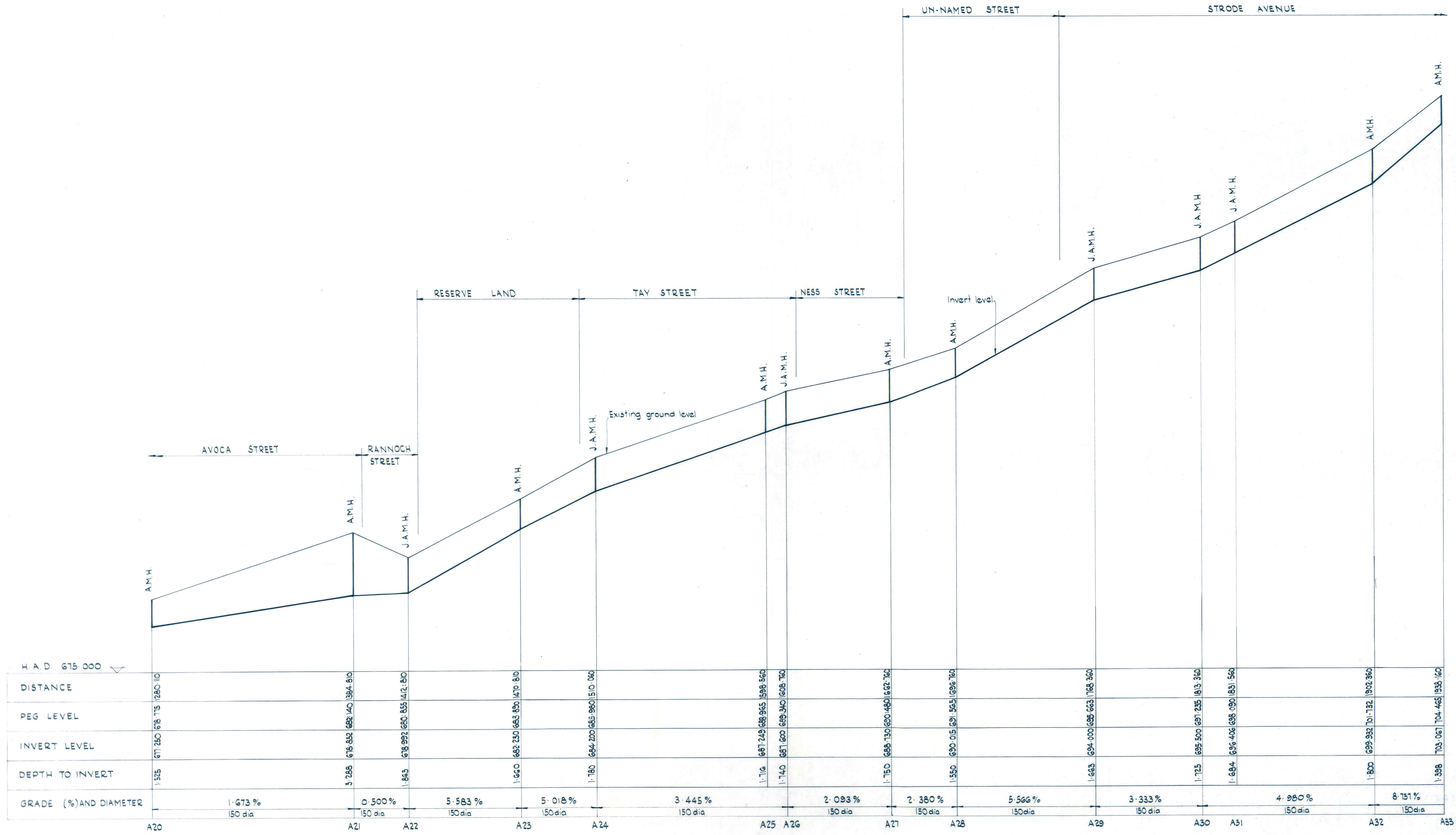
PROFILES Scales - Horizontal 1:1000 Vertical 1:100
