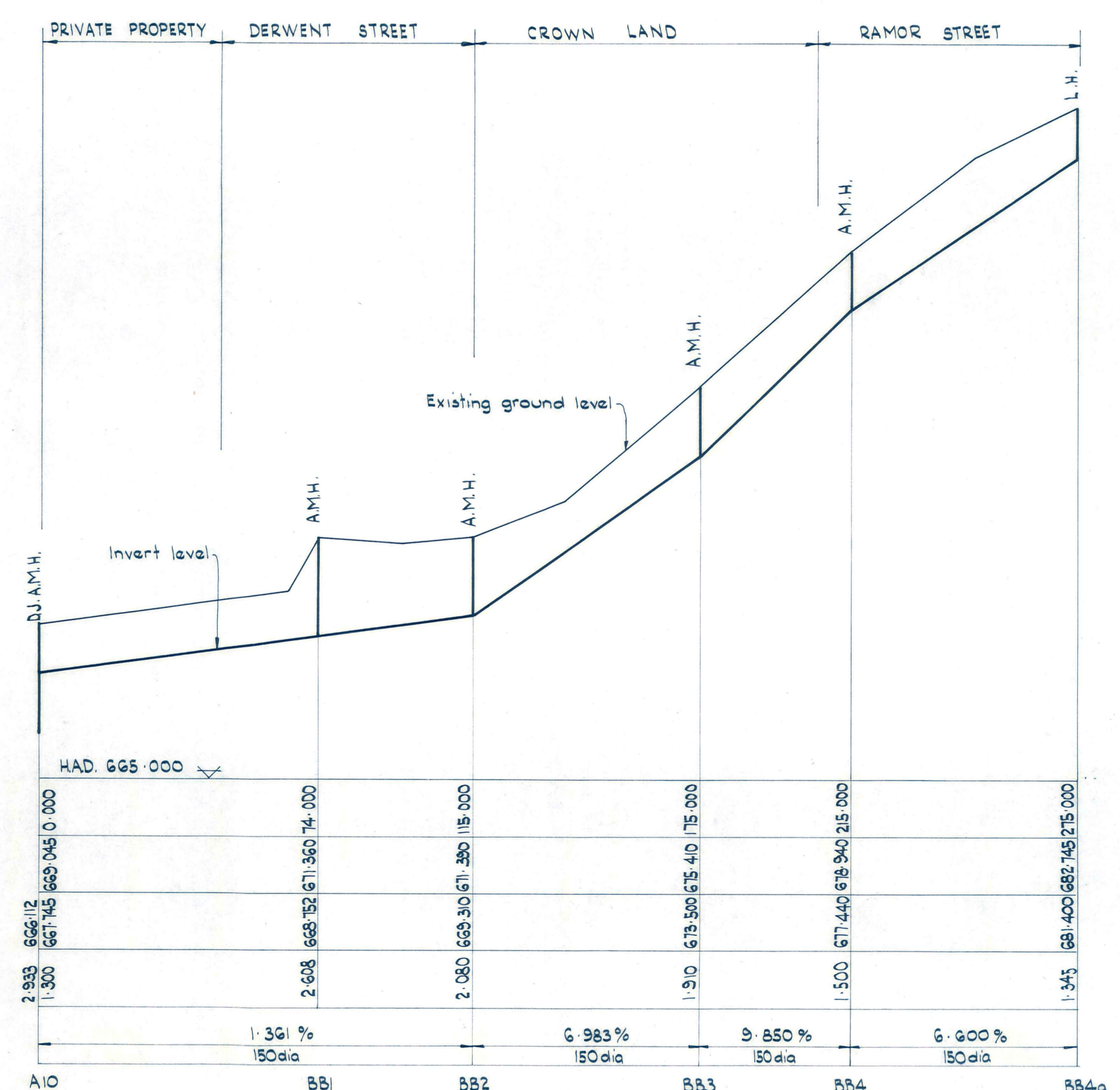
PROFILES Scales - Horizontal 1:1000 Vertical 1:100
