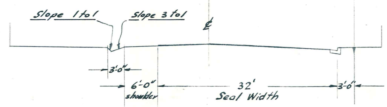
TYPICAL X-SECTION
