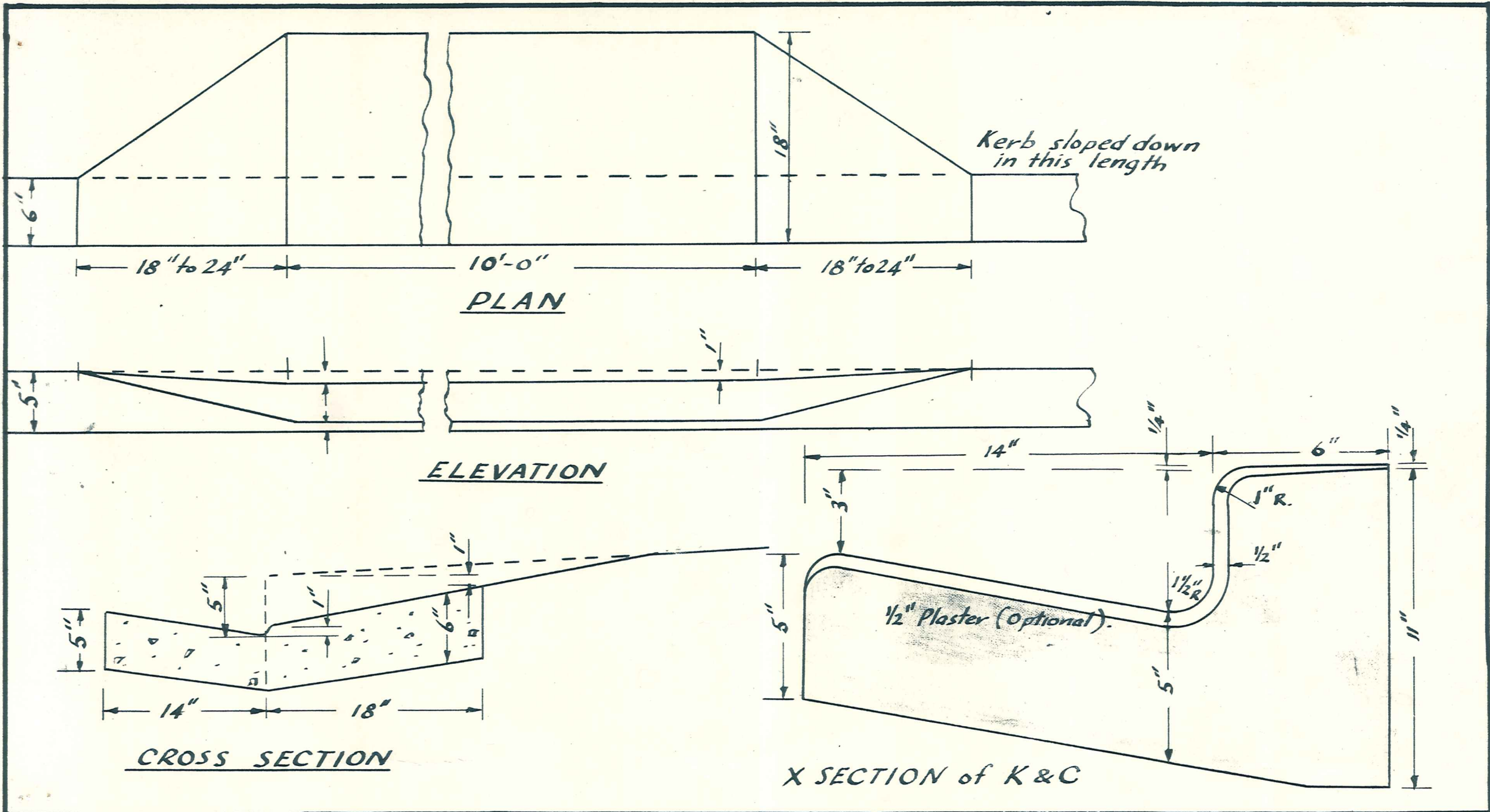
STANDARD KERB & CHANNEL & KERB CROSSING
