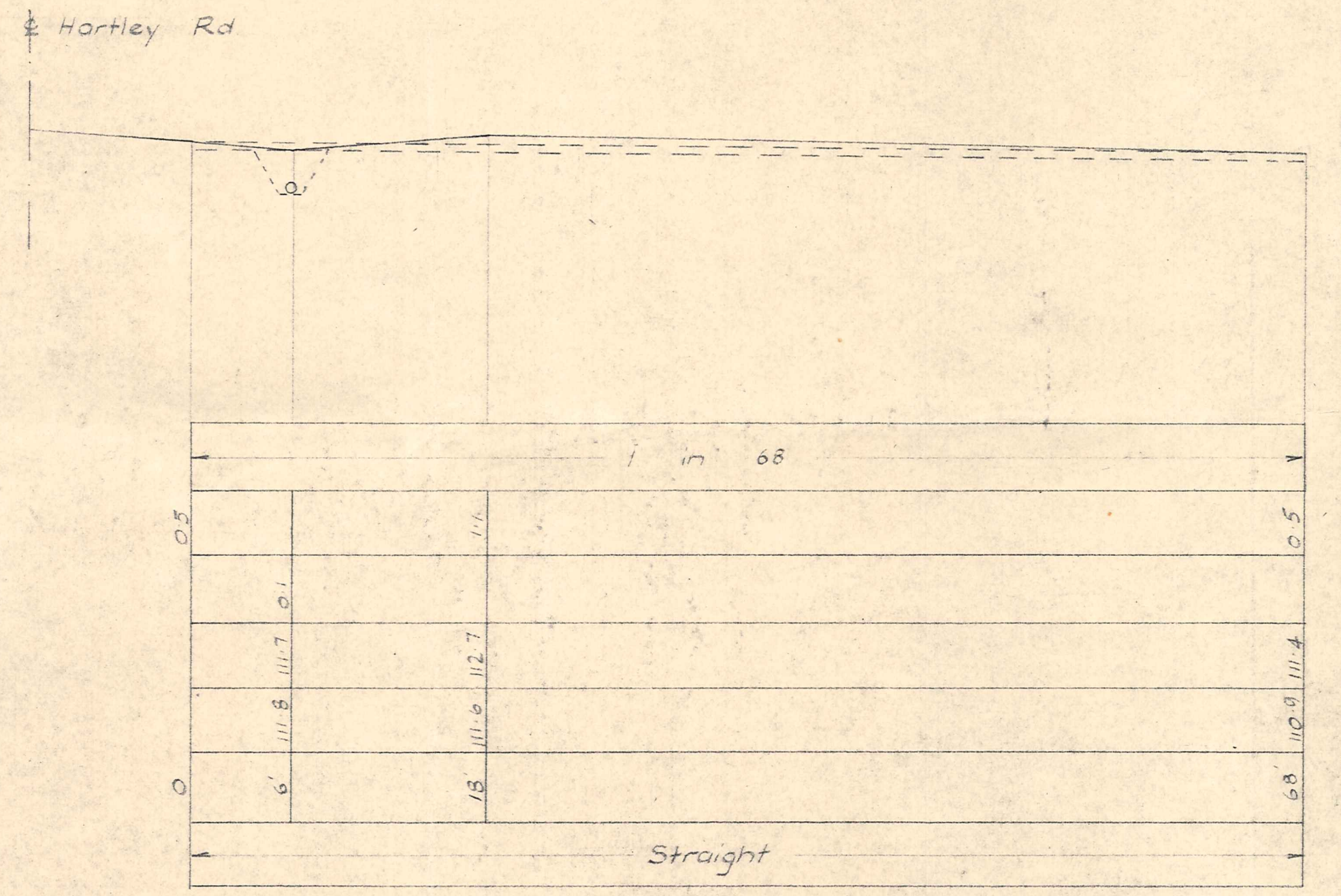
LONGITUDINAL SECTION ON £ CUL DE SAC ROAD Scale 1/8" = 1'-0"
