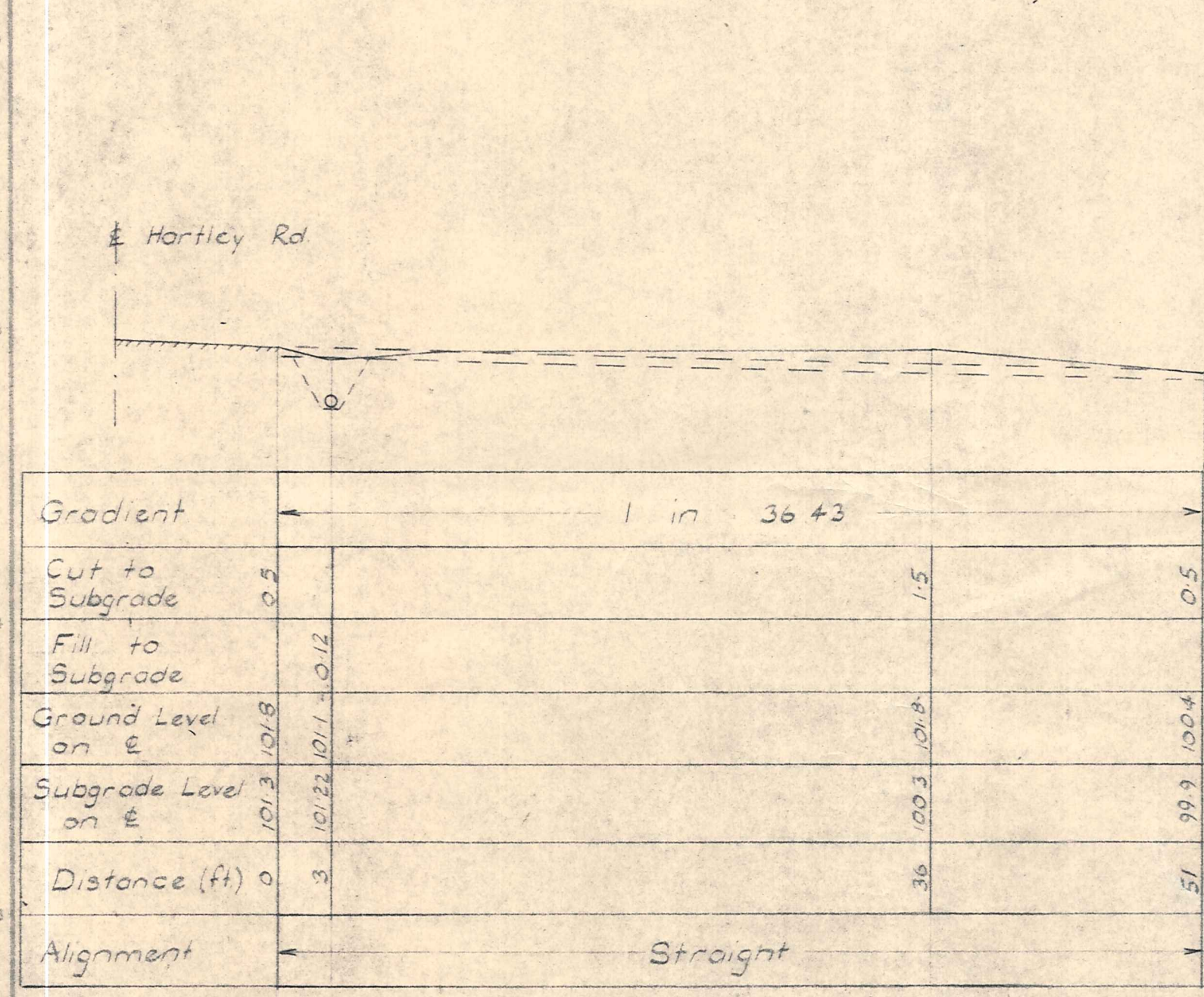
LONGITUDINAL SECTION ON £ SM CAMP ACCESS ROAD Scale 1/8" = 1'-0"
