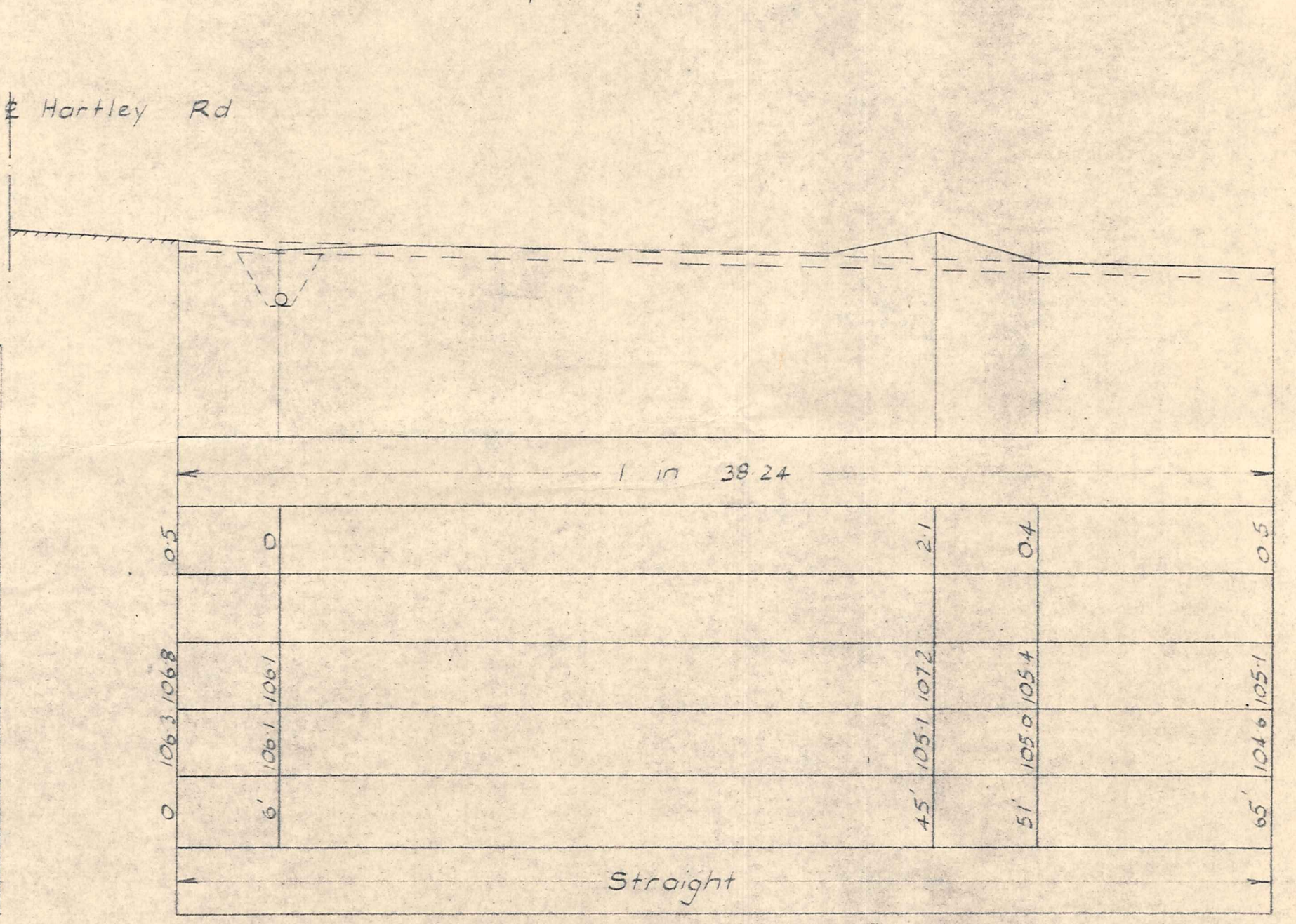
LONGITUDINAL SECTION ON £ MAIN ACCESS ROAD Scale 1/8" = 1'-0"
