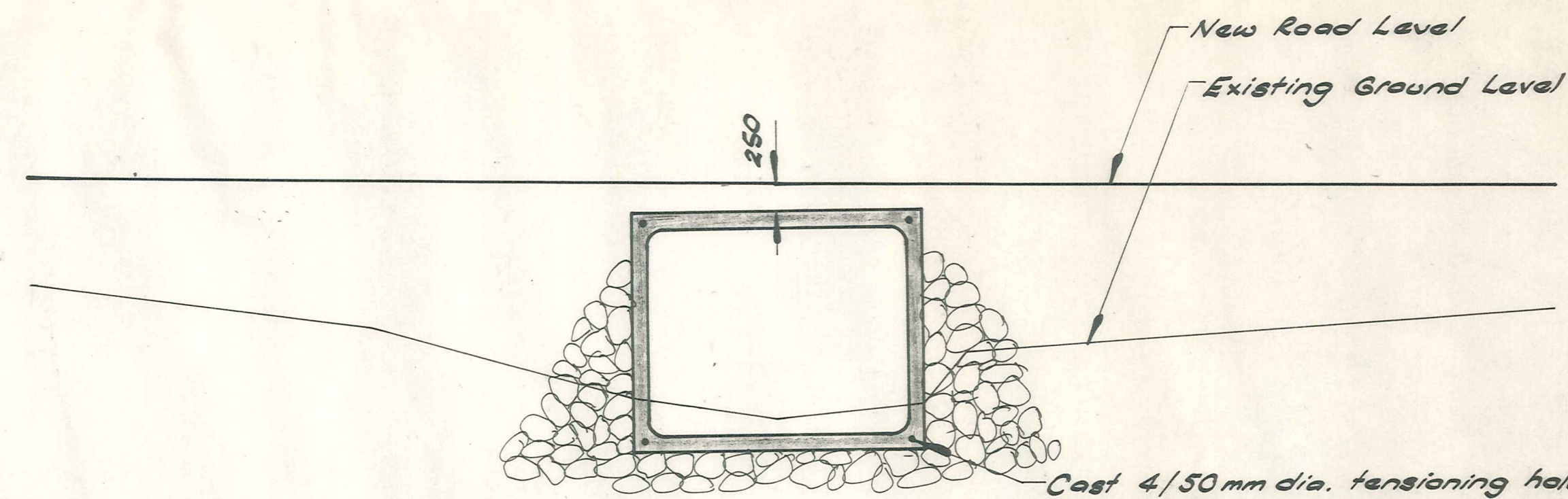
CROSS SECTION ON BRIDGE C
