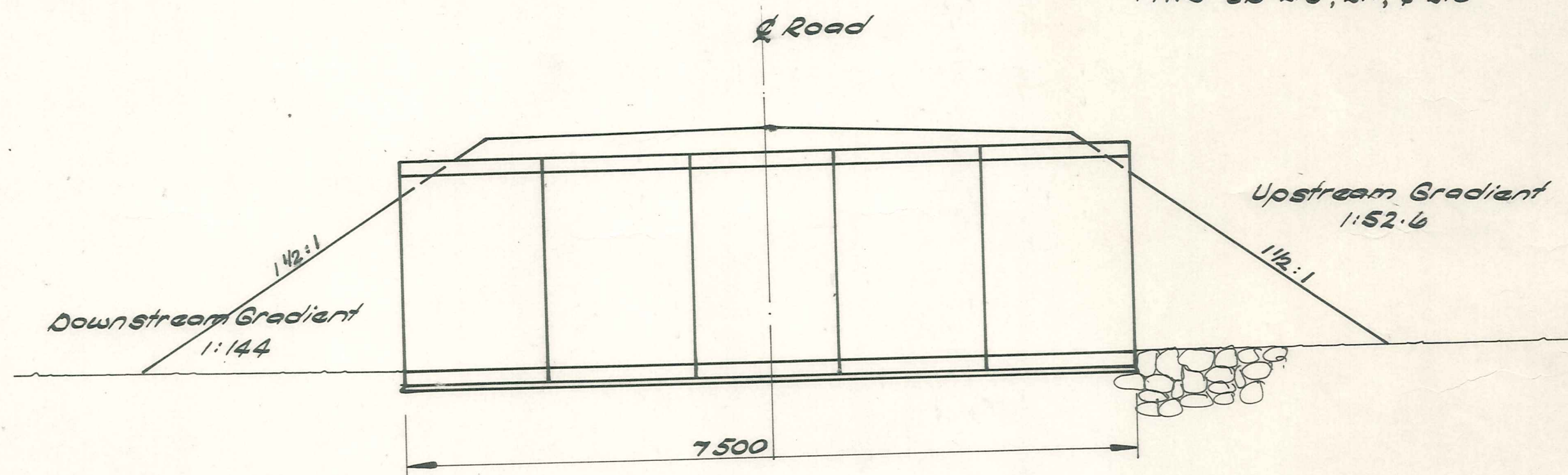
CROSS SECTION ON CULVERT D 1:50
